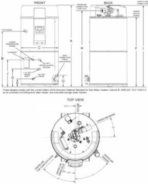
Figure 5. Rough-In Dimensions
