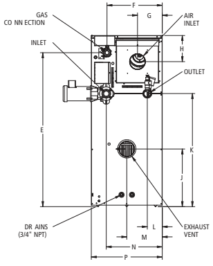
REAR VIEW (VWH1500N-VWH2000N)
